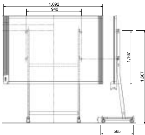
Dimensions* with Optional Stand
