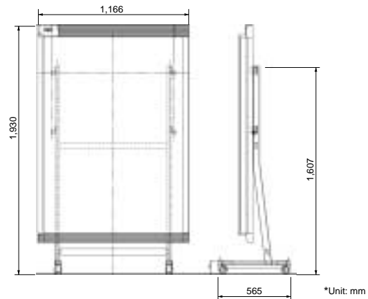
Dimensions* with Optional Stand (when in moving position)
